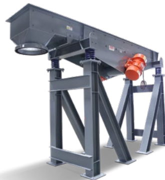
Sand Feeder
